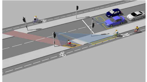
Dual Zone / Active Travel (Cycle Lane Detection)
